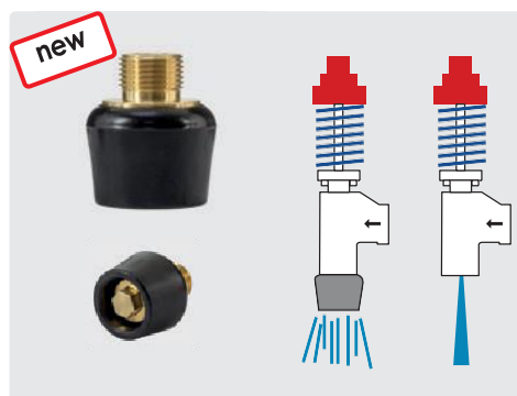
Jetbreaker
